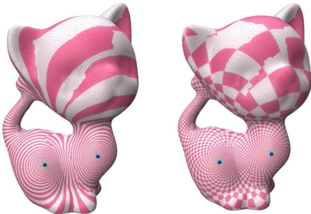
(图 17: 带极点的调和叶状结构和亚纯二次微分, Geometric 作图。) (Figure 17: A harmonic foliation and its meromorphic quadratic differential.)
